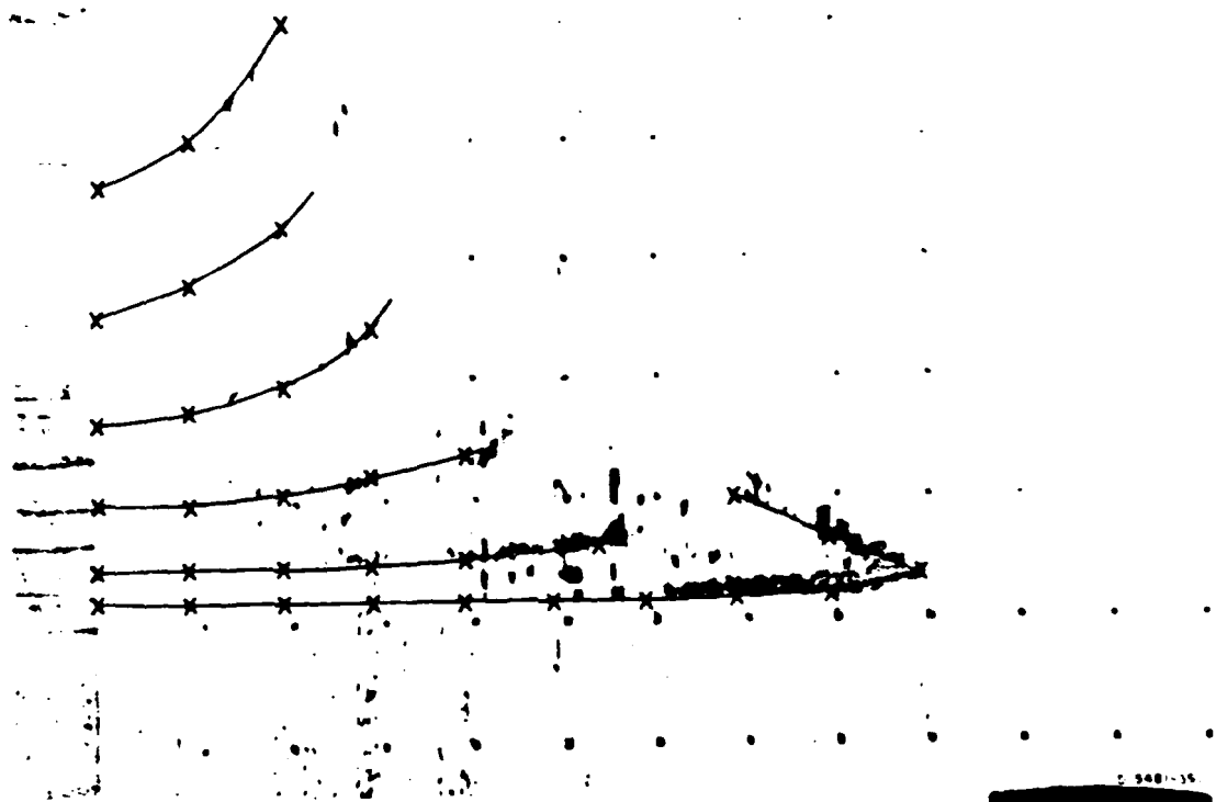
FIGURE 3-4 █ CALCULATED AND MEASURED IONOGRAM FOR OKINAWA TO SAIGON PATH
